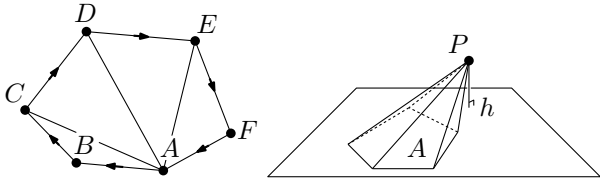
Fig. 5. Left: decomposition of a convex polygon into triangles to compute its area. Right: decomposition of a convex polyhedron into pyramids to compute its volume.
