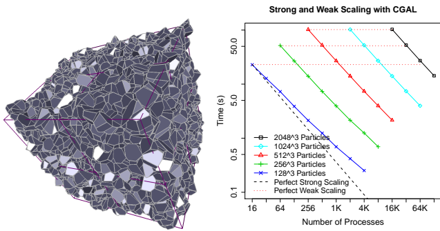
Fig. 7. Left: Voronoi tessellation of synthetic data using 16^3 particles and 8 blocks. Right: strong and weak scaling (excluding I/O time) using CGAL for a particle counts ranging from 128^3 up to 2048^3 . Processor counts range from 16 to 128K.
