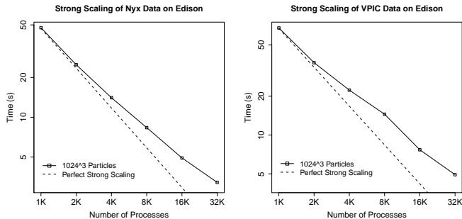
Fig. 9. Left: Strong scaling (excluding I/O time) using CGAL for a Nyx middle time step of 1024^3 particles. Right: Same for one time step of VPIC data.
