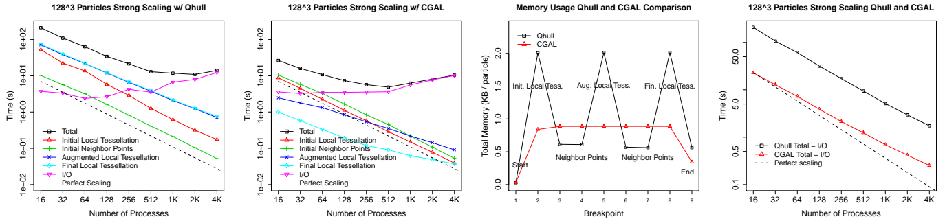
Fig. 6. Strong scaling for 128^3 particles tessellated in parallel using Qhull (far left) and CGAL (center left). Total time is further broken down into main component times. Center right: total memory usage during the execution of the algorithm normalized by the number of particles. Far right: strong scaling (excluding I/O time) comparison between Qhull and CGAL for 128^3 particles.
