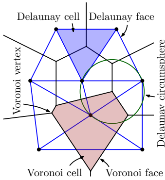
Fig. 1. Voronoi and Delaunay tessellation nomenclature. Input points are black dots. Voronoi tessellation is illustrated with black edges. Delaunay tessellation is in blue. A Voronoi cell is highlighted with a red shaded polygon. A Delaunay cell is highlighted with a blue shaded triangle. An empty Delaunay circumisphere is shown in green.
