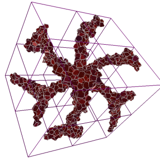
Fig. 10. Voronoi cells of the A species of the double gyroid. The sixfold “wheel” structure formed by the A domain is characteristic of the double gyroid phase.
