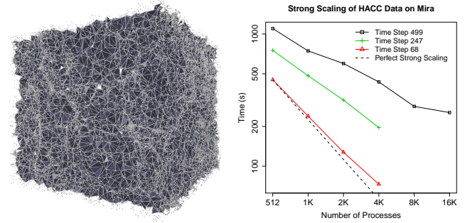
Fig. 8. Left: Delaunay tessellation of 128^3 dark matter tracer particles. Right: strong scaling (excluding I/O time) using CGAL for three time steps of HACC data of 1024^3 particles.
