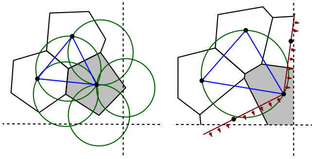
Fig. 2. Left: Circumspheres at vertices of a finite Voronoi cell. Right: An infinite Voronoi cell and the half-spaces supported by the facets of the convex hull. The edges of the blocks are shown by dotted lines.
