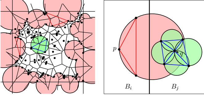
Fig. 3. Left: The green Delaunay circumcircle is contained entirely in the local block, and therefore the blue triangle remains Delaunay in the final triangulation. The red circumcircles intersect other blocks; the triangles they circumscribe are not yet finalized. Right: Despite the fact that point q falls into an (unfinished) circumcircle supported by point p , we don't need to send it to block B_j since its surrounding circumcircles are finalized (empty of any points).
